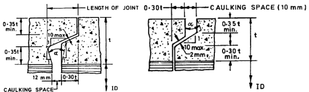
Internal flush Joint
