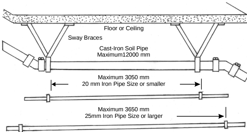
Location of C.I. Hangers for C.I. Pipes
