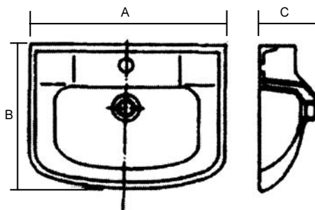
Flat back wash basin (I.S.2556-Pt.4)
