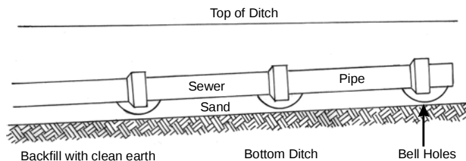
Support for Under Ground Pipe
