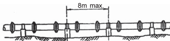
Pipes above normal level
