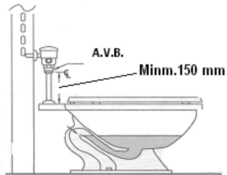
Flusho-meter valve Location (A.V.B.)
