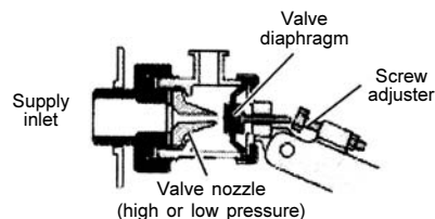
Diaphragm valve
