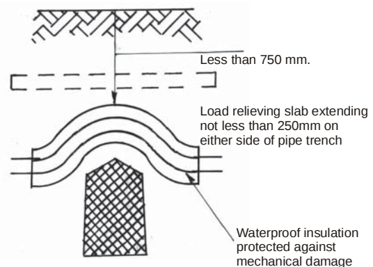
Pipe laid over an obstruction
