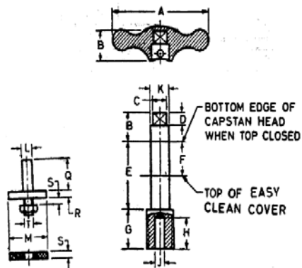
Spindle of pillar tap
