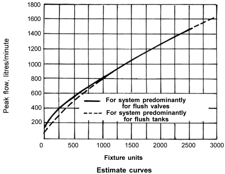
Graph for assessing the flow in litre/min.
