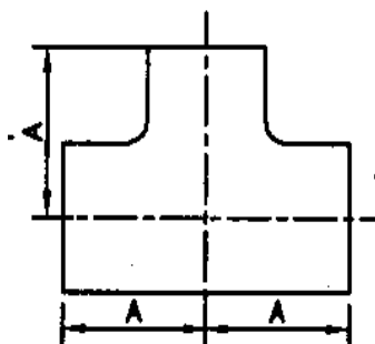
TEE, EQUAL
