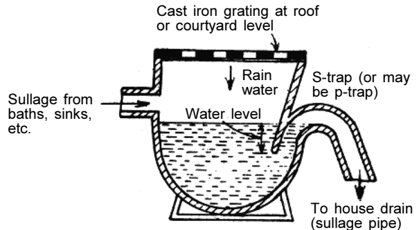
Gully trap
