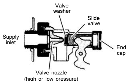
Slide valve
