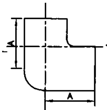
ELBOW, EQUAL
