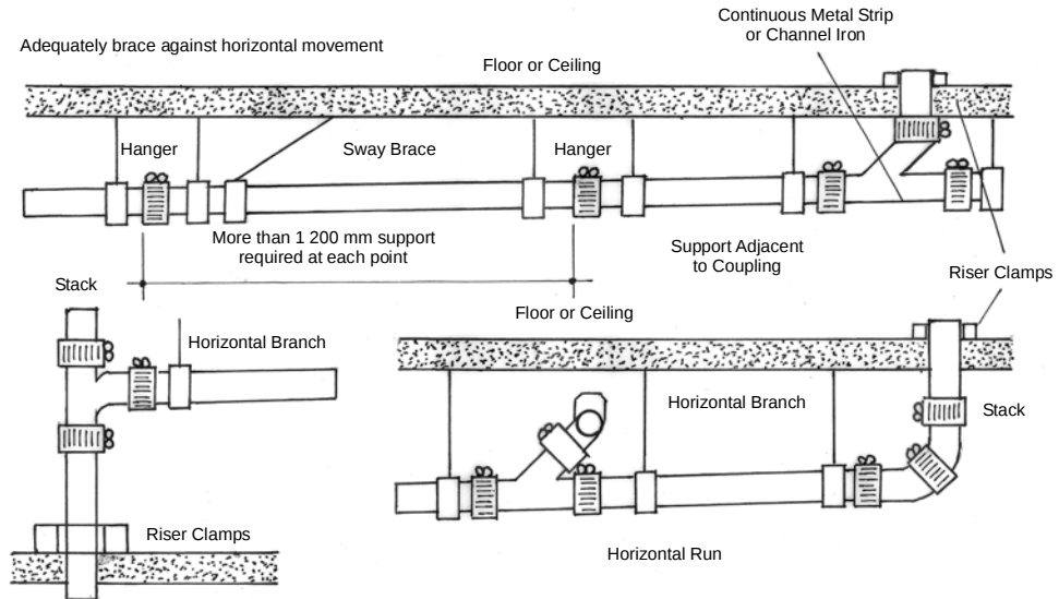
Location of C.I. Hangers for C.I. Pipes
