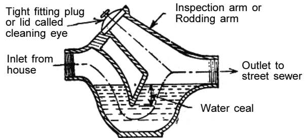
Intercepting trap
