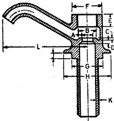
Body of pillar tap
