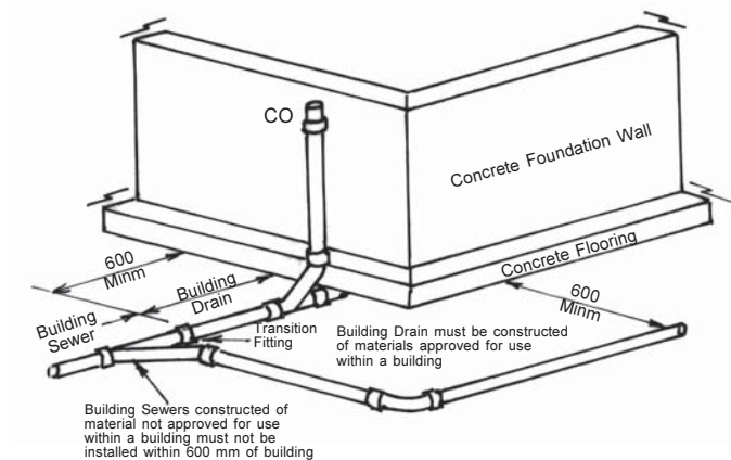
Required clearances for piping materials used for building drain and building sewers
