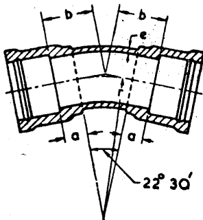
Bend 22.5°
