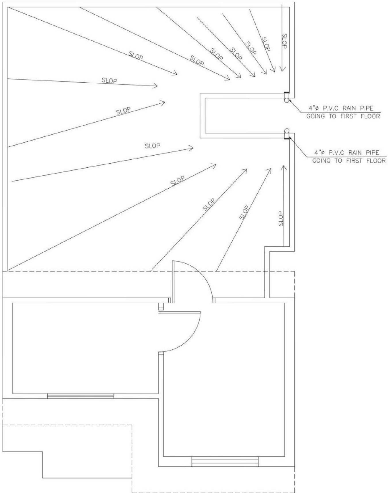
○ SEWERAGE PLAN (SECOND Floor)
